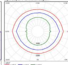
Light output 1/ luminance diagram
