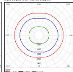
Light output 1 / luminance diagram
